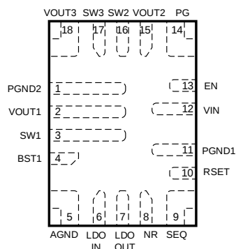
Top View: 18-Lead FCTOFN 2.5mmx3.5mm
