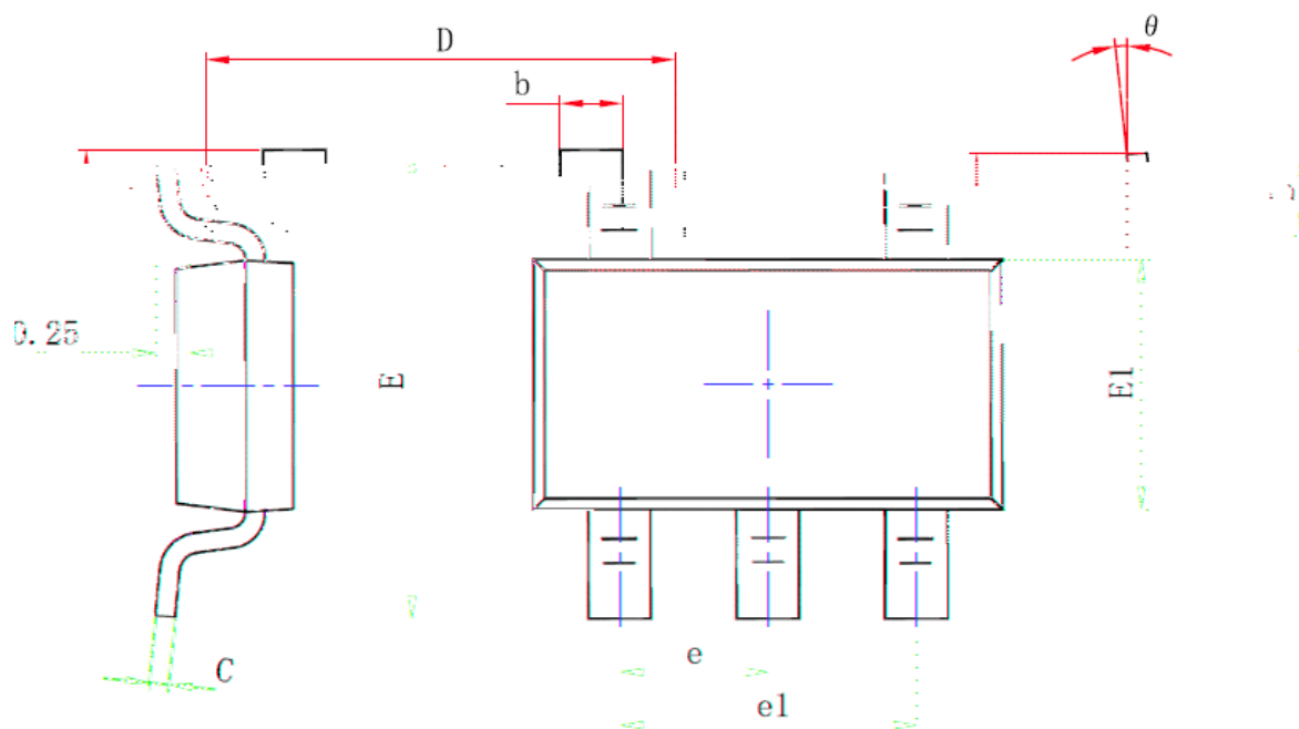
TOP VIEW
