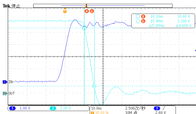
Figure 19. IN- Switching OFF( T_F )
